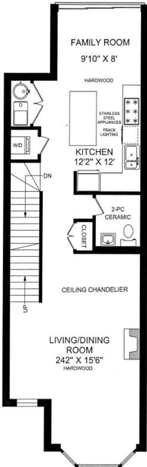
MAIN LEVEL 822 SQUARE FEET (CEILING HEIGHT : 9'-0")
