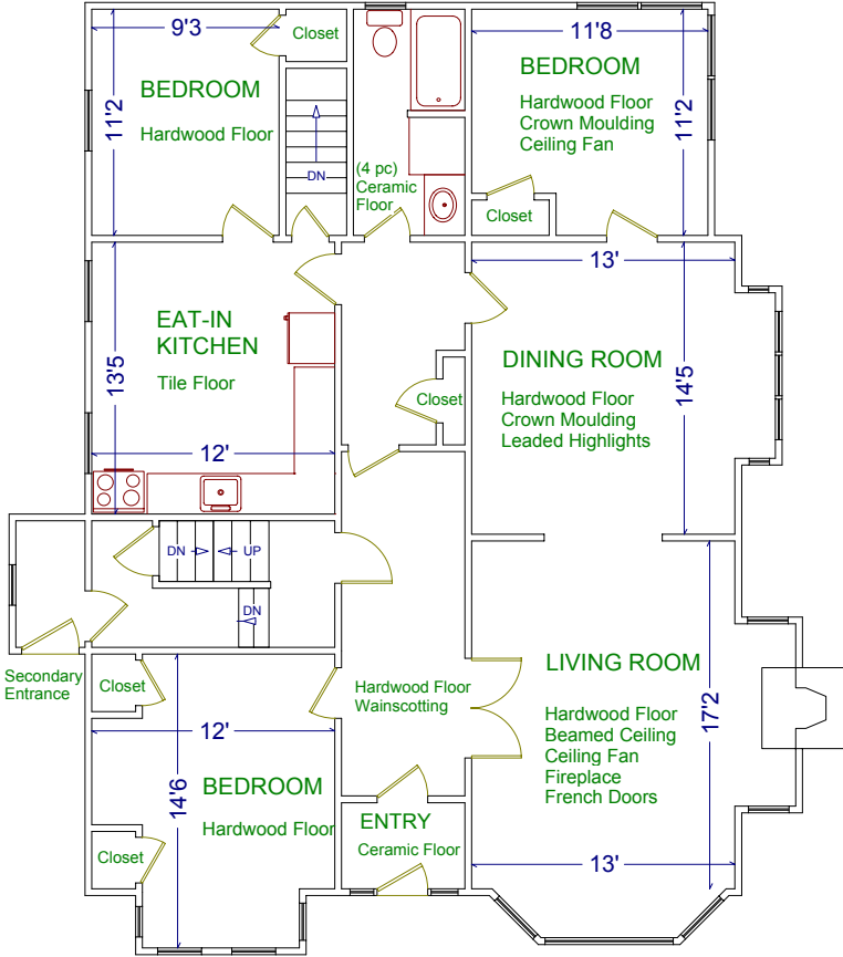
MAIN FLOOR (1,510 sq ft)
