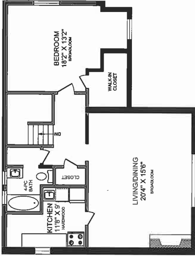
THIRD FLOOR 957 SQUARE FEET (CEILING HEIGHT : 8'-0")
