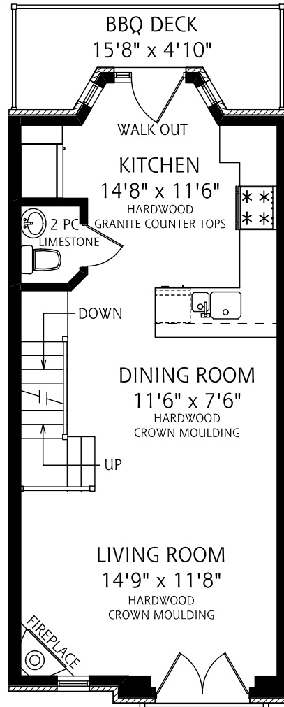
MAIN LIVING FLOOR 560 SQUARE FEET
