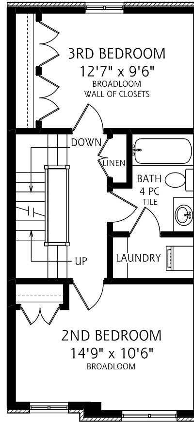
BEDROOMS FLOOR 550 SQUARE FEET
