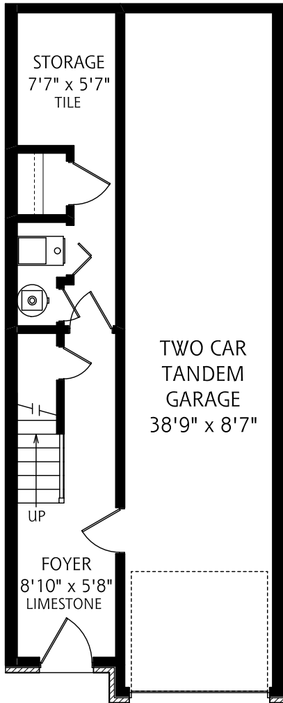
GROUND ENTRY FLOOR 265 SQUARE FEET
