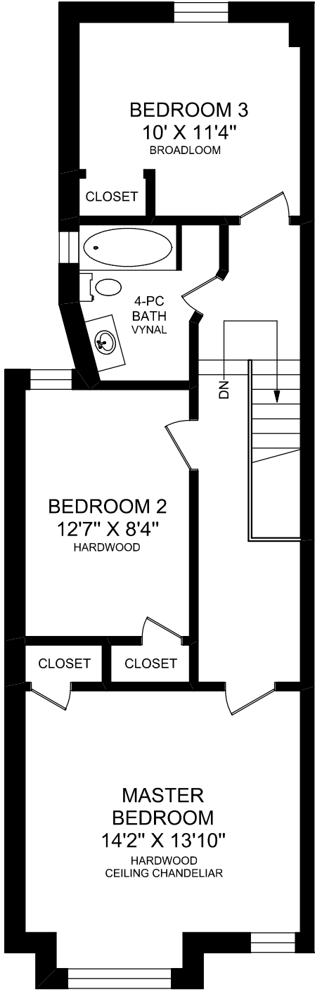
SECOND FLOOR 724 SQUARE FEET (CEILING HEIGHT : 9'-0")
