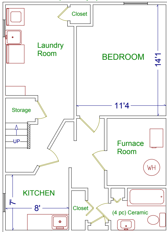
BASEMENT (615 sq ft)
