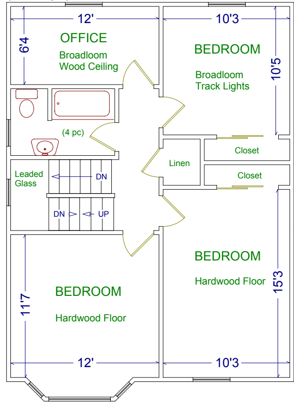
THIRD FLOOR (590 sq ft)
