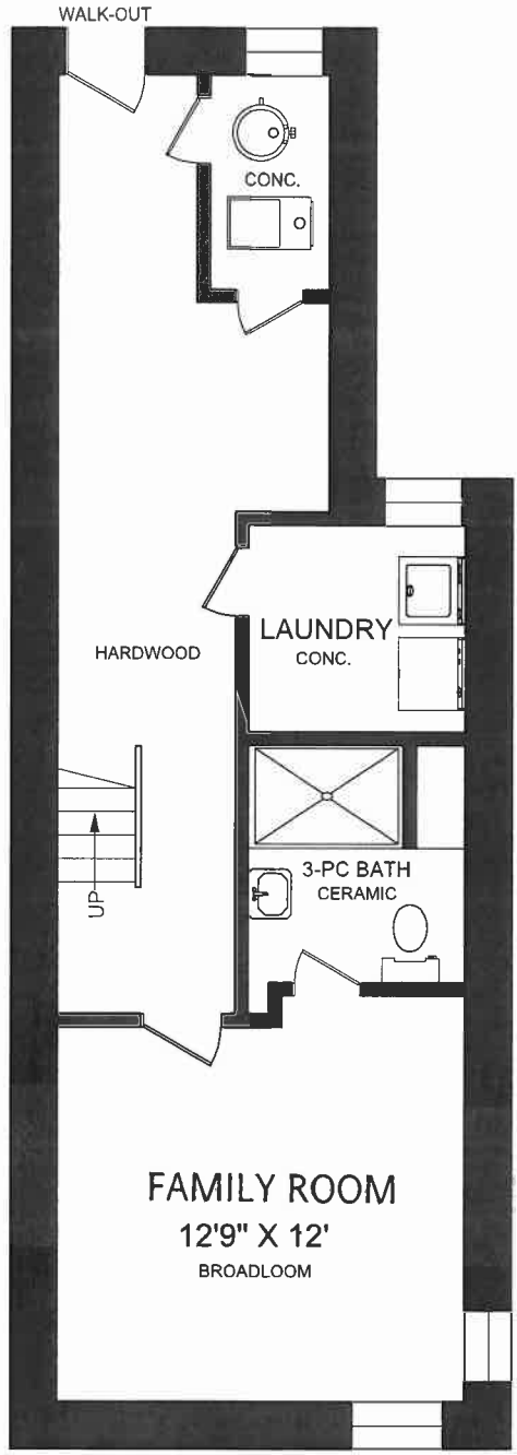
LOWER LEVEL 673 SQUARE FEET (CEILING HEIGHT : 6'-9")
