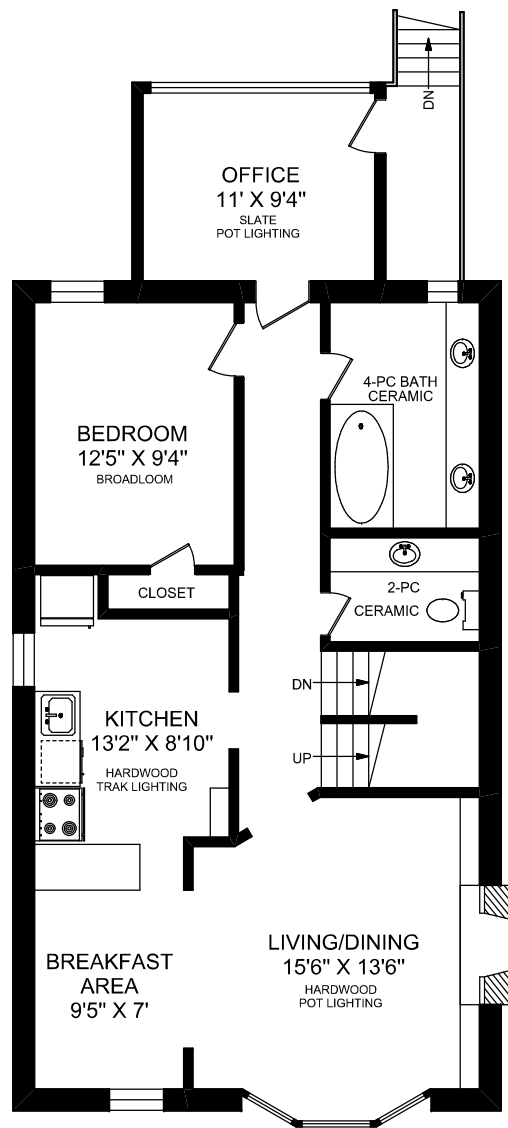
SECOND FLOOR 1018 SQUARE FEET (CEILING HEIGHT : 8'-4")
