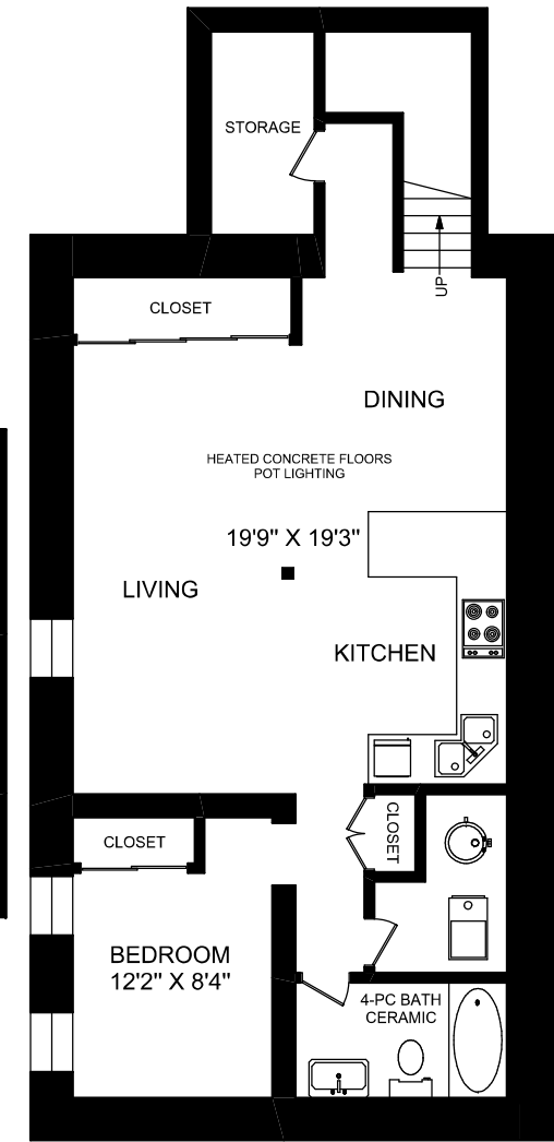
LOWER LEVEL 1033 SQUARE FEET (CEILING HEIGHT : 6'-10")
