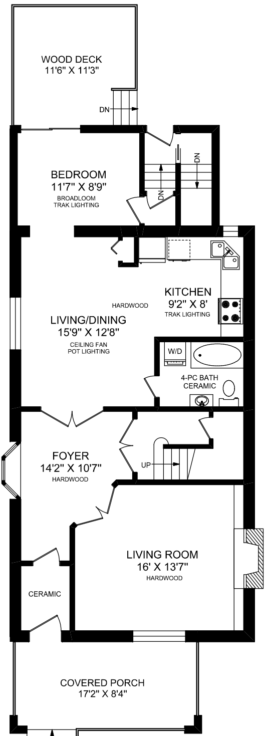
MAIN FLOOR 1092 SQUARE FEET (CEILING HEIGHT : 9'-2")
