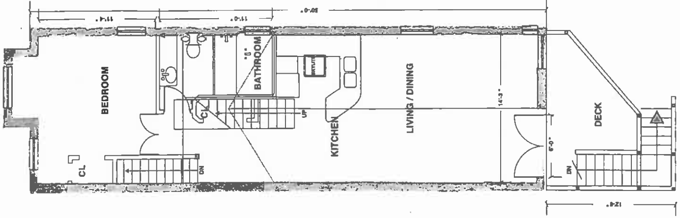
SECOND FLOOR 720 SQUARE FEET
