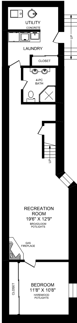
LOWER LEVEL 1067 SQUARE FEET (CEILING HEIGHT : 7'-0")
