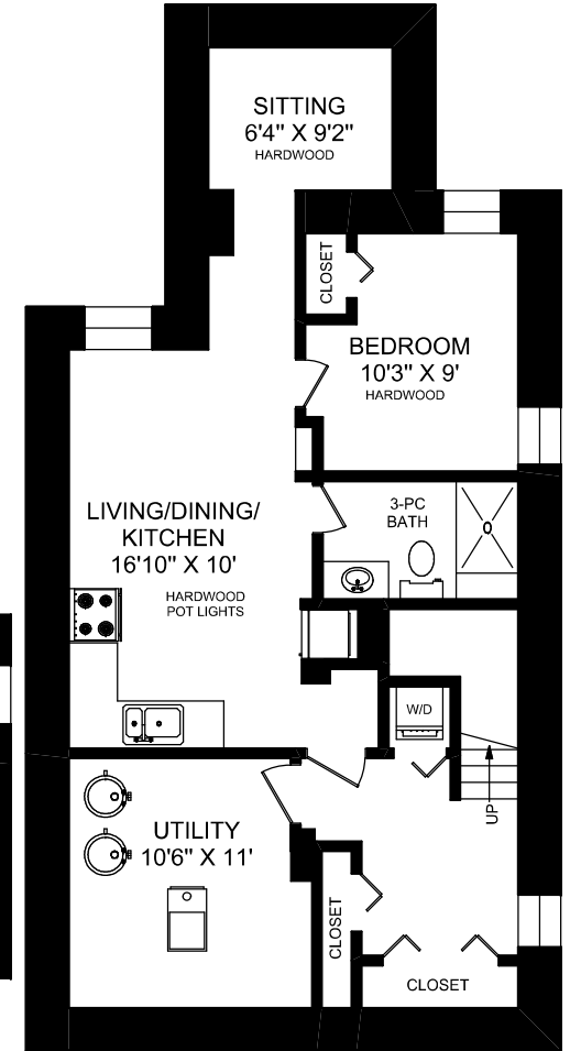
LOWER LEVEL 912 SQUARE FEET (CEILING HEIGHT : 6'-6")
