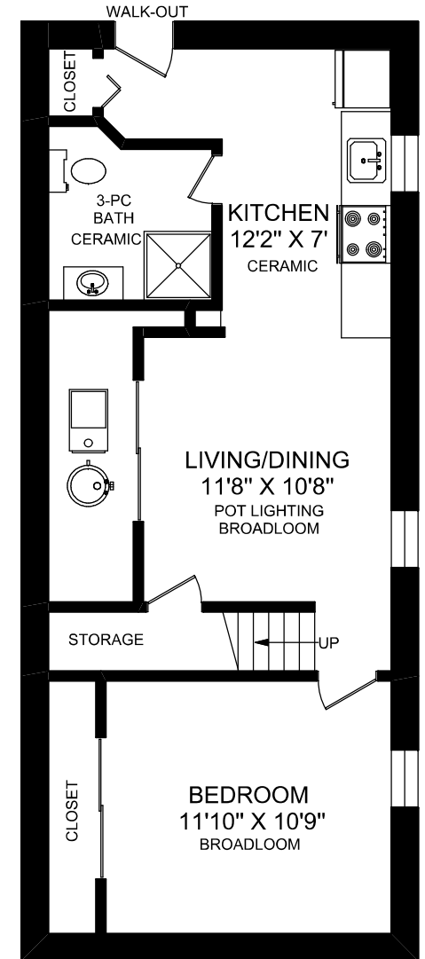
LOWER LEVEL 703 SQUARE FEET (CEILIG HEIGHT : 6'-10")
